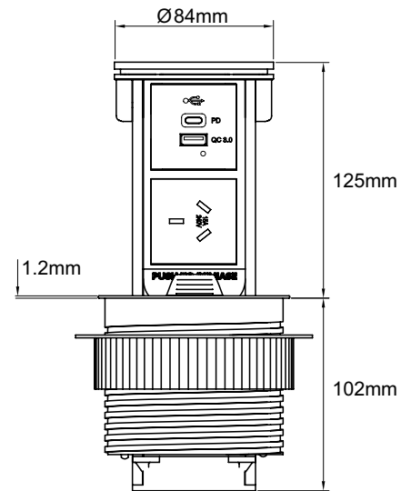
Flush Pop Up Duo
