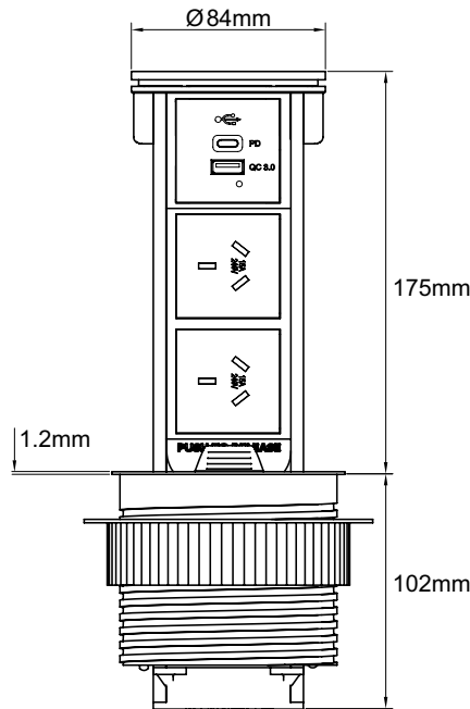
Flush Pop Up Trio
