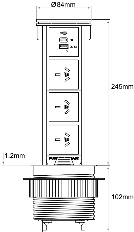
Flush Pop Up Quad
